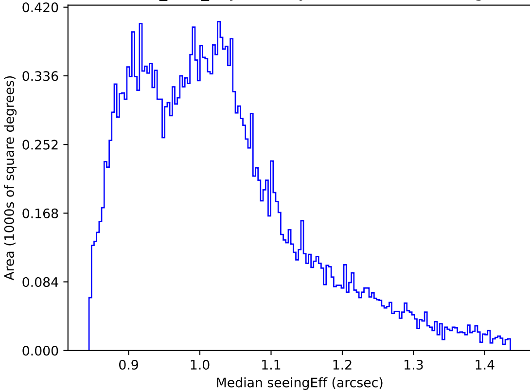
baseline_v3.0_10yrs All sky i band: Median seeingEff
