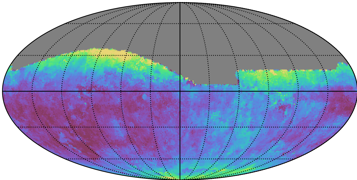
baseline_v3.0_10yrs All sky g band: Median seeingEff
