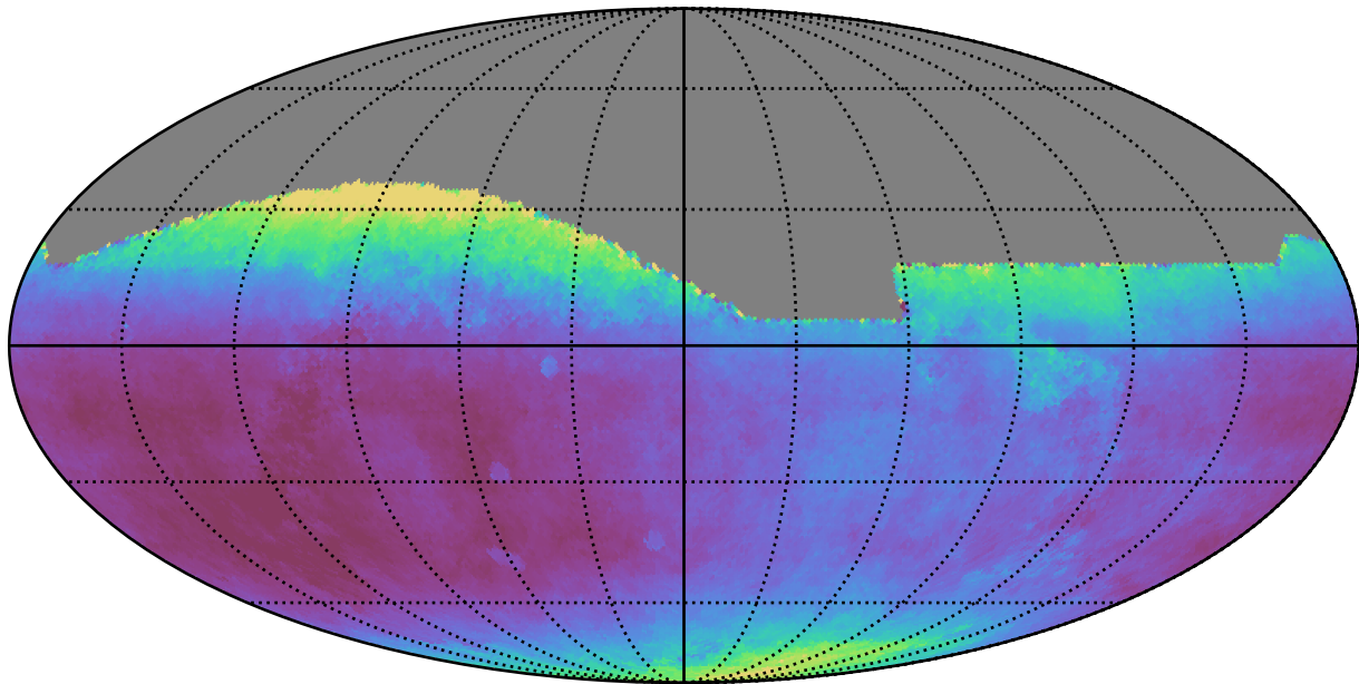
baseline_v3.0_10yrs All sky all bands: Median seeingEff
