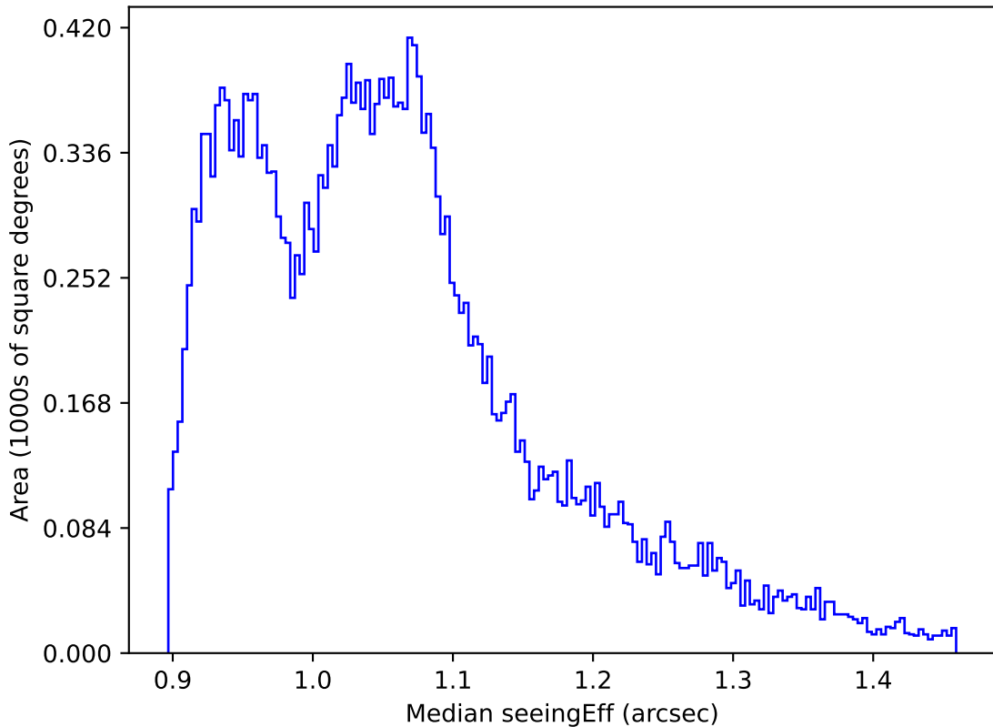
baseline_v3.0_10yrs All sky all bands: Median seeingEff
