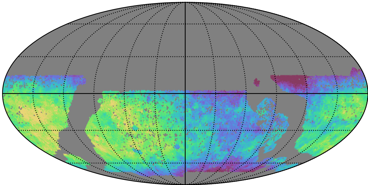
baseline_v3.0_10yrs WFD z band: Median saturation_mag
