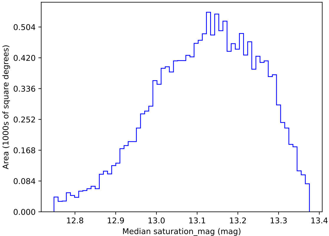
baseline_v3.0_10yrs WFD y band: Median saturation_mag
