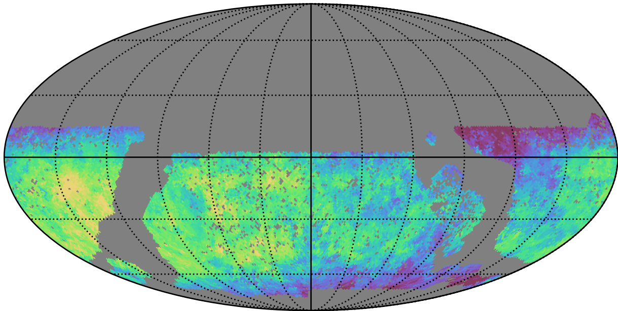
baseline_v3.0_10yrs WFD u band: Median saturation_mag
