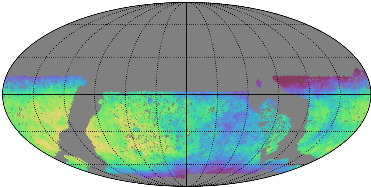
baseline_v3.0_10yrs WFD r band: Median saturation_mag
