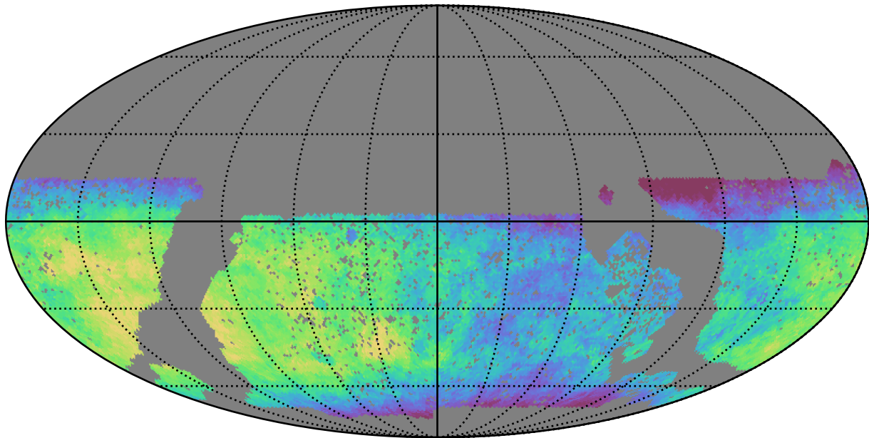
baseline_v3.0_10yrs WFD i band: Median saturation_mag
