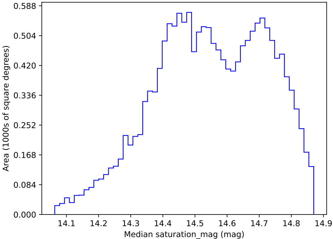
baseline_v3.0_10yrs WFD i band: Median saturation_mag
