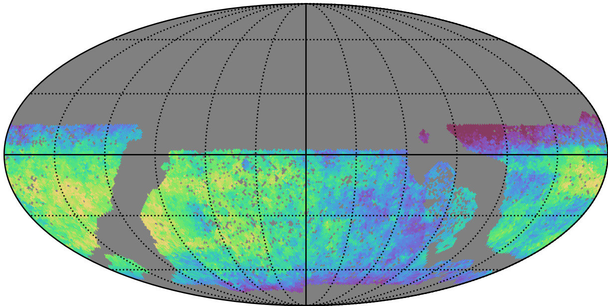
baseline_v3.0_10yrs WFD g band: Median saturation_mag
