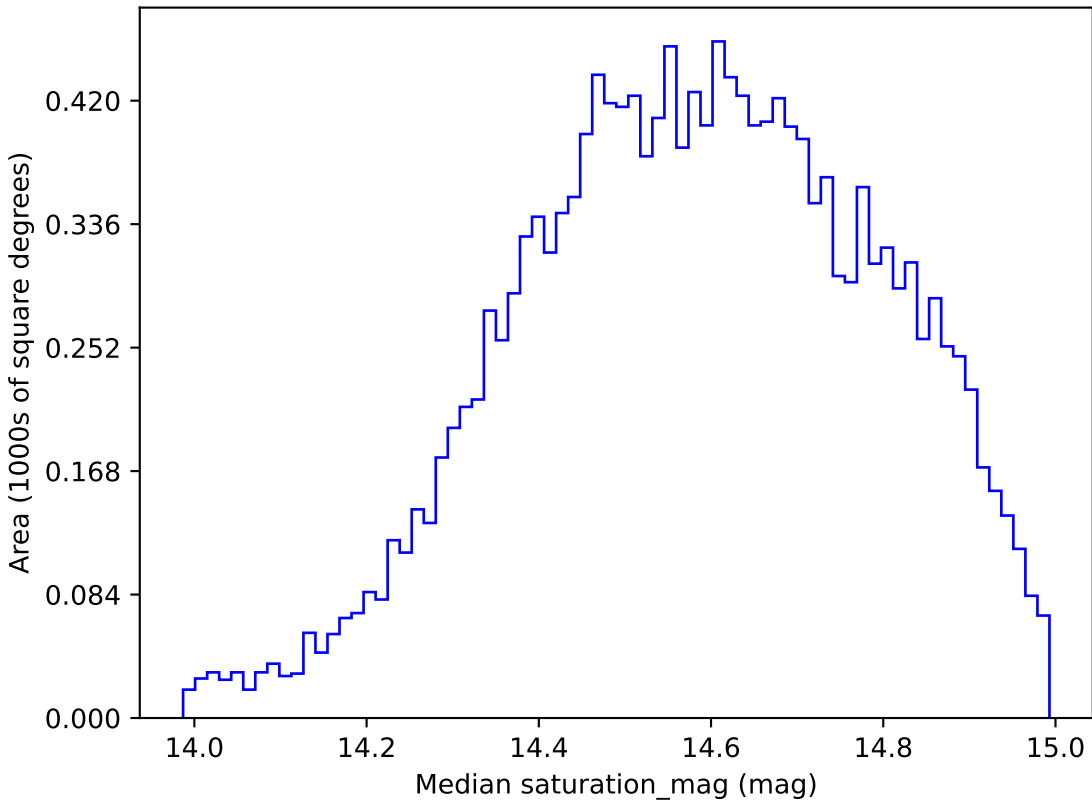
baseline_v3.0_10yrs WFD g band: Median saturation_mag
