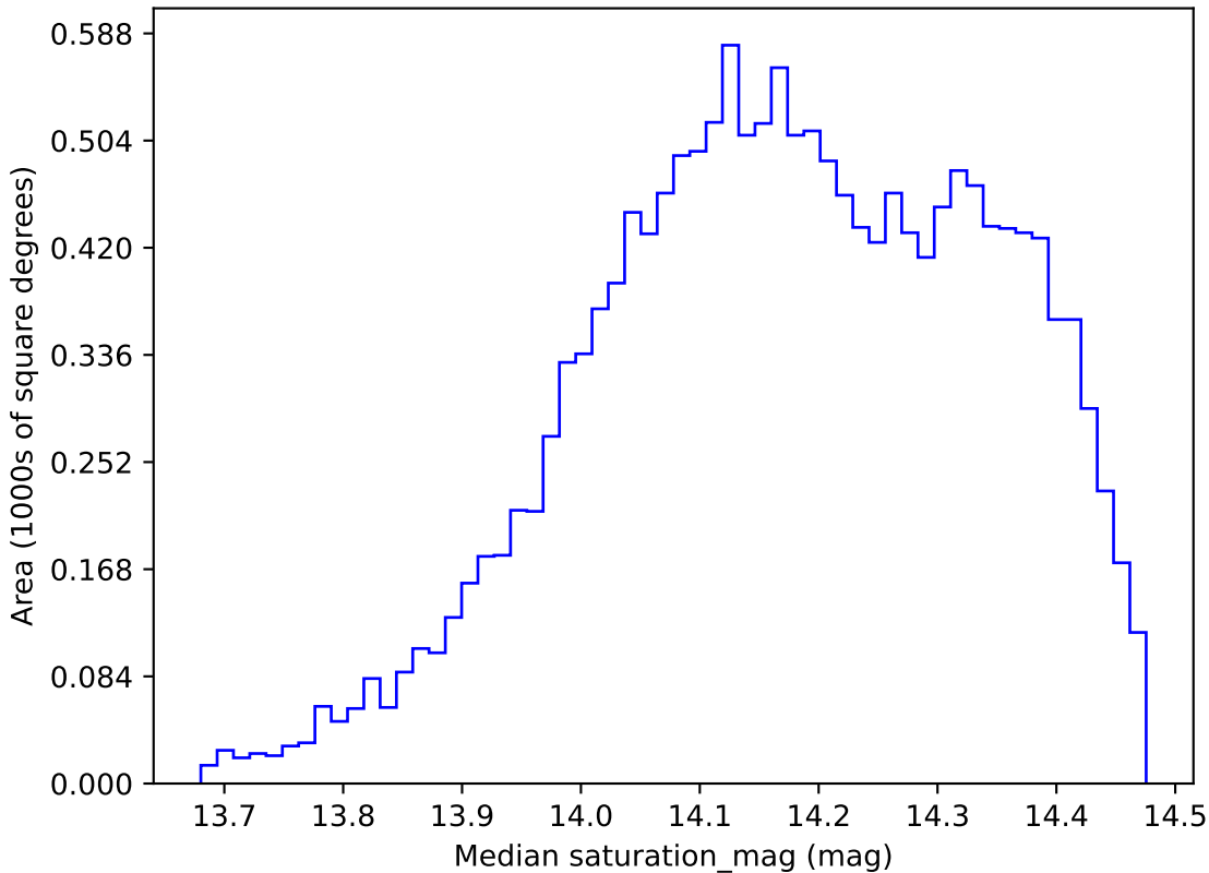
baseline_v3.0_10yrs WFD all bands: Median saturation_mag
