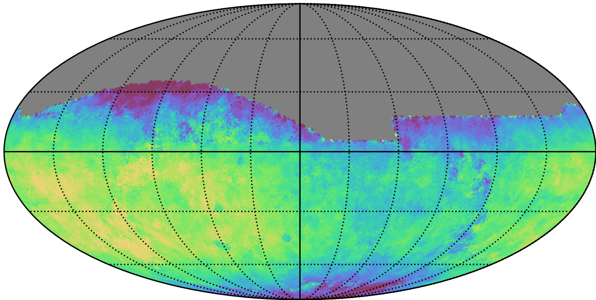
baseline_v3.0_10yrs All sky z band: Median saturation_mag
