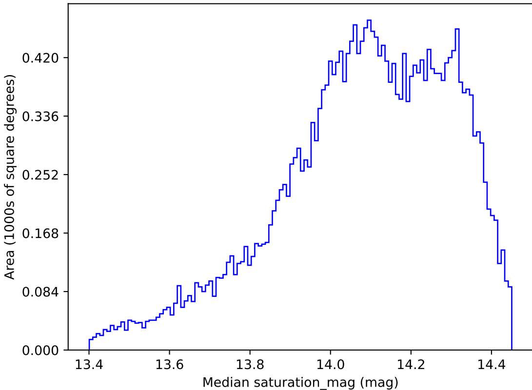
baseline_v3.0_10yrs All sky z band: Median saturation_mag
