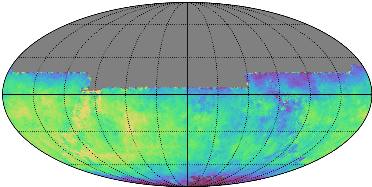
baseline_v3.0_10yrs All sky y band: Median saturation_mag
