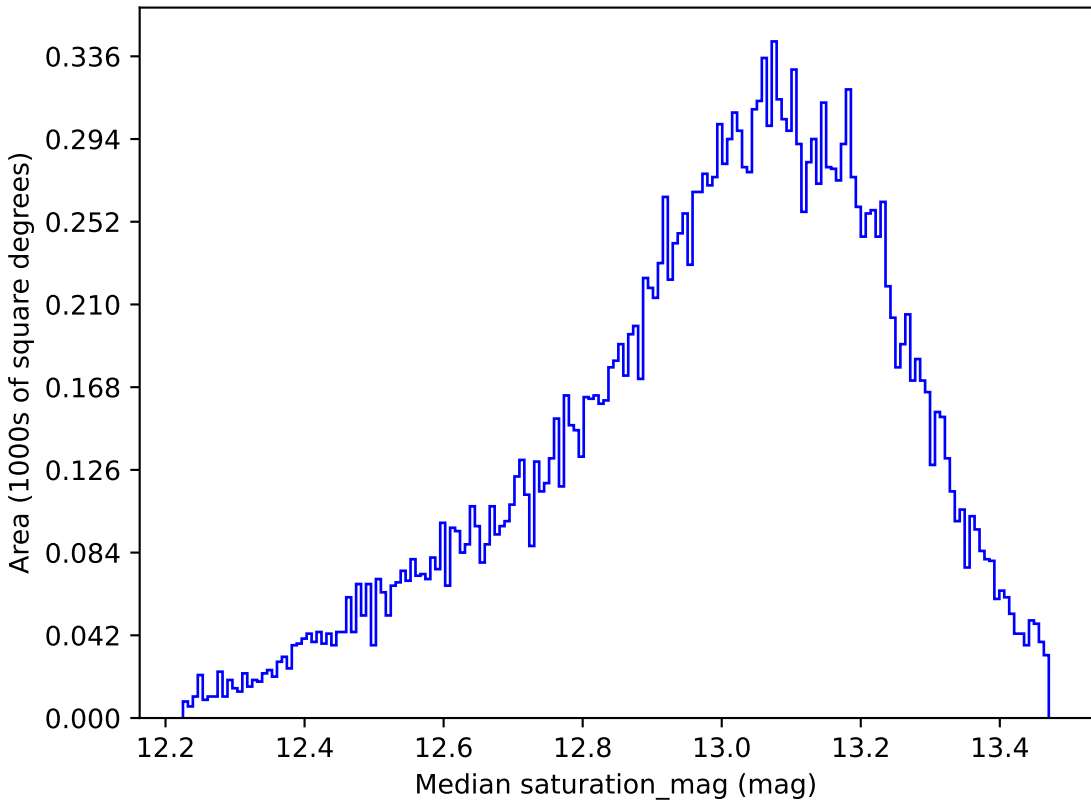
baseline_v3.0_10yrs All sky u band: Median saturation_mag
