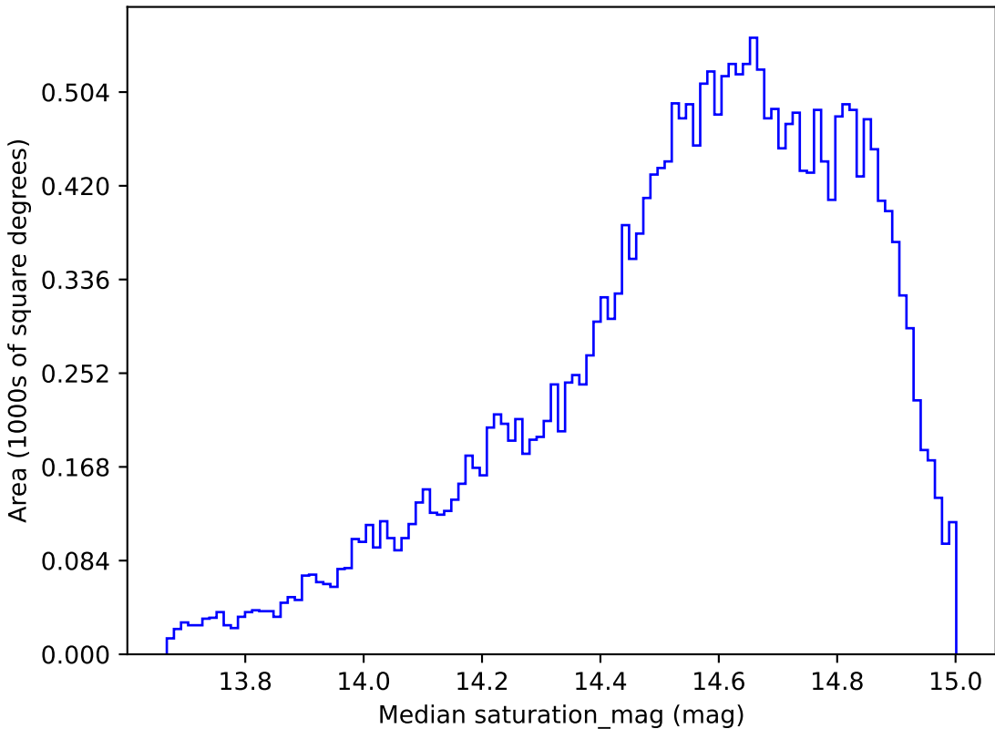
baseline_v3.0_10yrs All sky r band: Median saturation_mag
