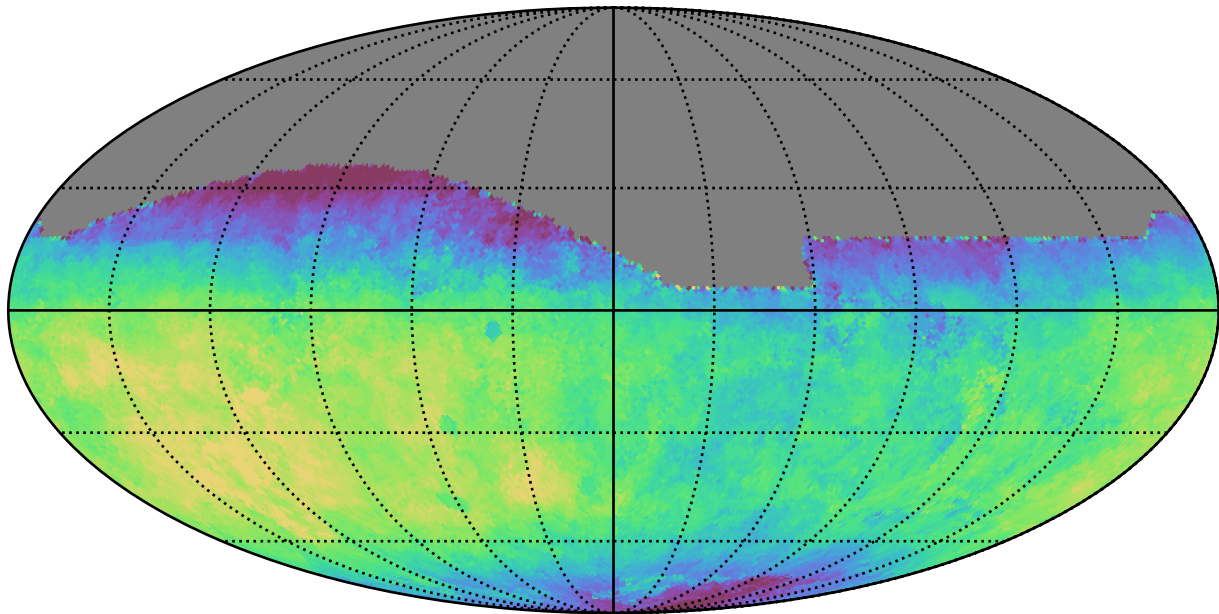
baseline_v3.0_10yrs All sky i band: Median saturation_mag
