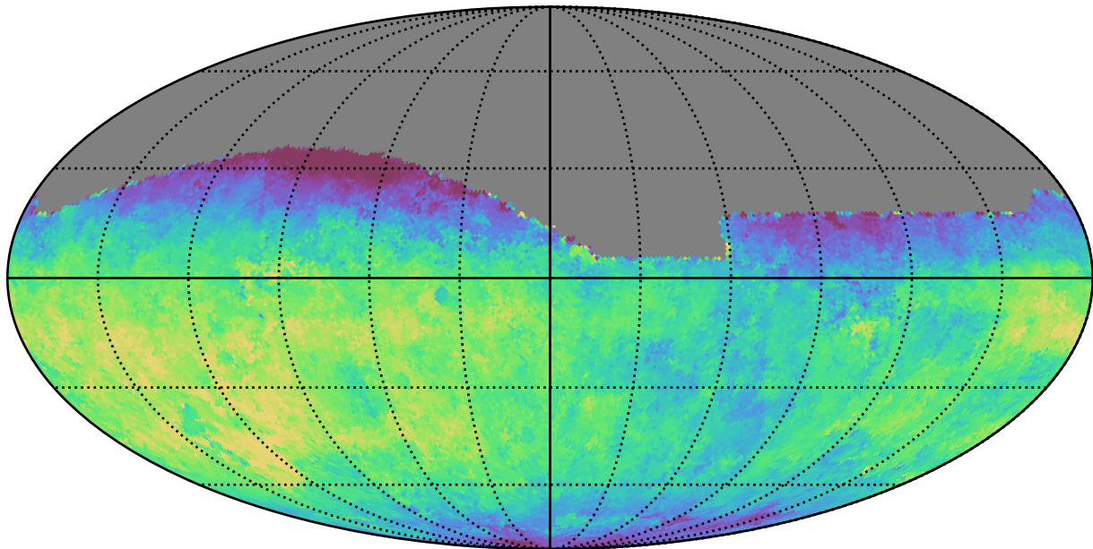
baseline_v3.0_10yrs All sky g band: Median saturation_mag
