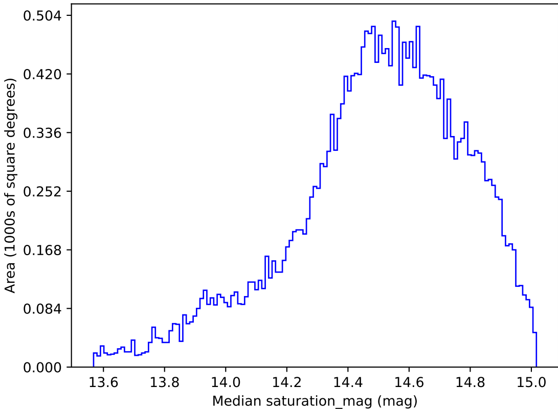
baseline_v3.0_10yrs All sky g band: Median saturation_mag
