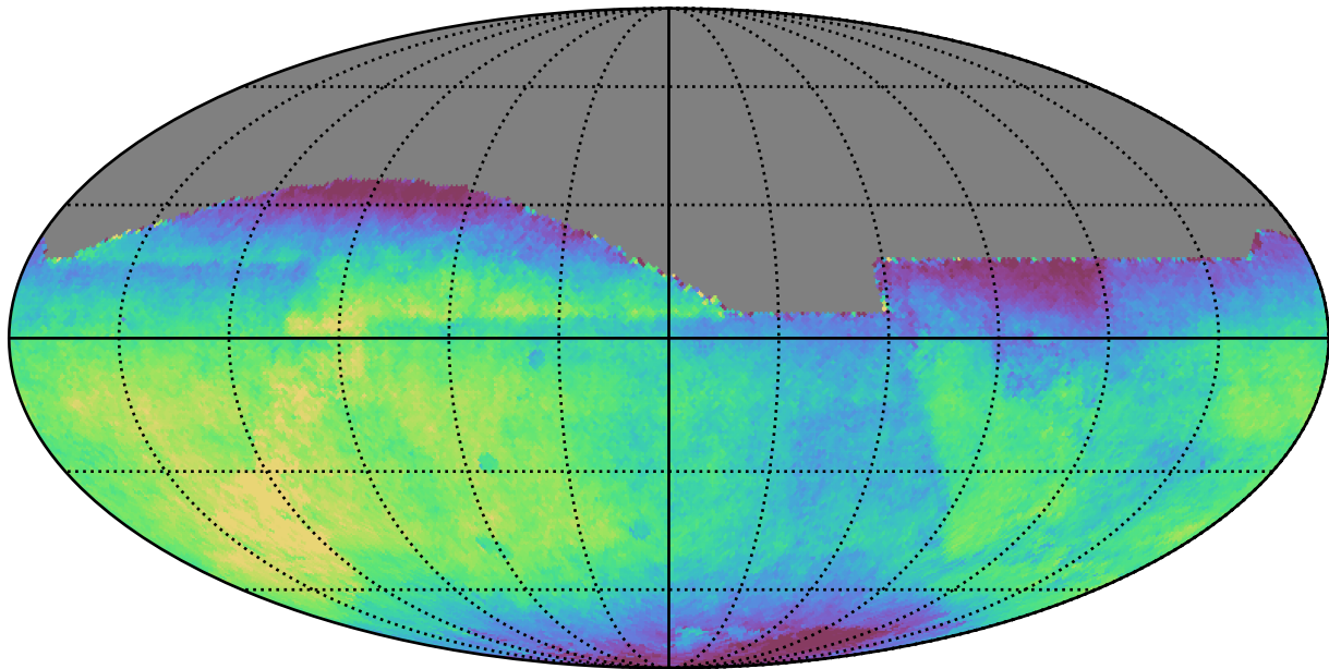
baseline_v3.0_10yrs All sky all bands: Median saturation_mag
