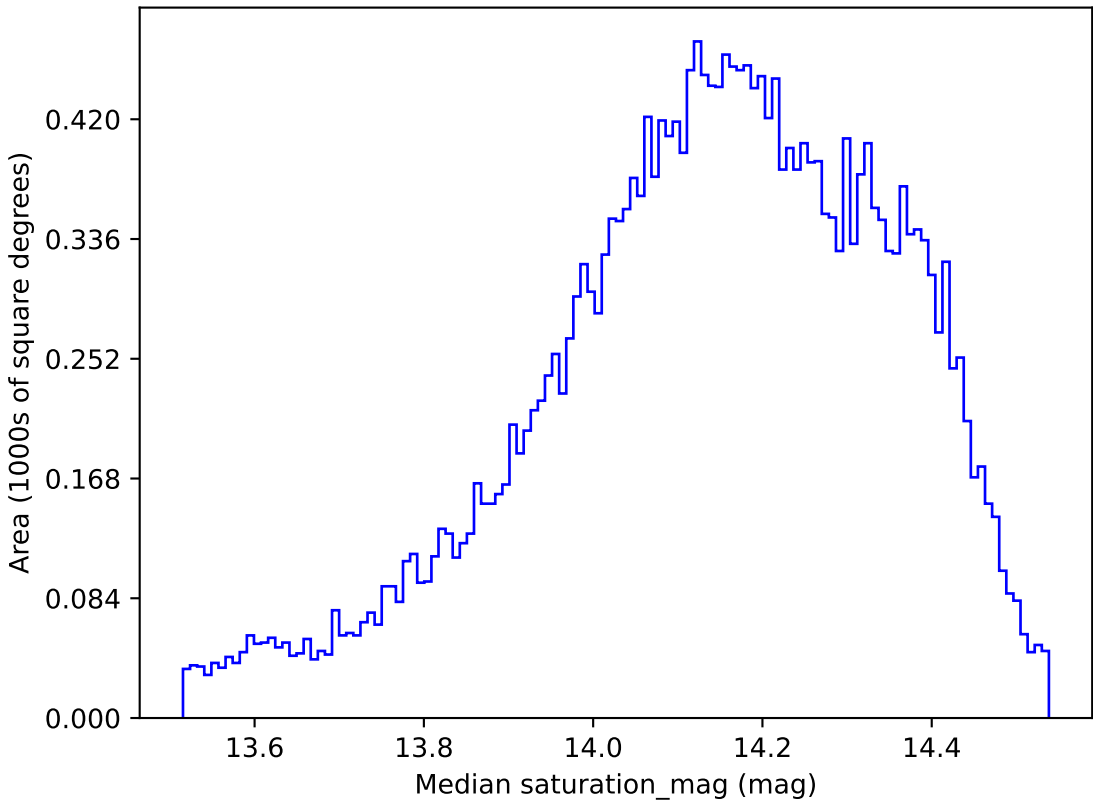
baseline_v3.0_10yrs All sky all bands: Median saturation_mag
