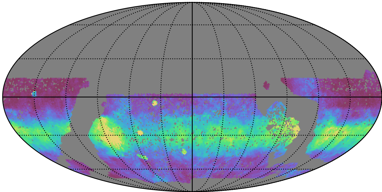
baseline_v3.0_10yrs WFD z band: Median normairmass
