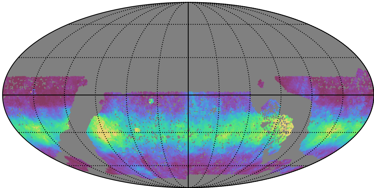
baseline_v3.0_10yrs WFD y band: Median normairmass
