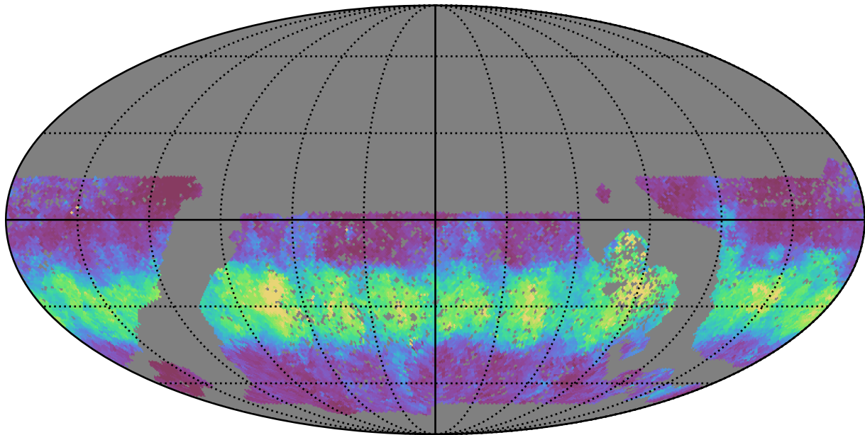
baseline_v3.0_10yrs WFD u band: Median normairmass
