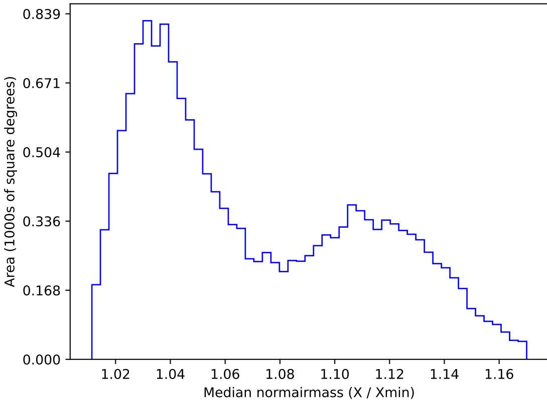
baseline_v3.0_10yrs WFD u band: Median normairmass
