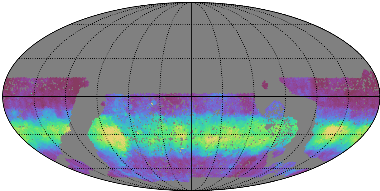
baseline_v3.0_10yrs WFD r band: Median normairmass
