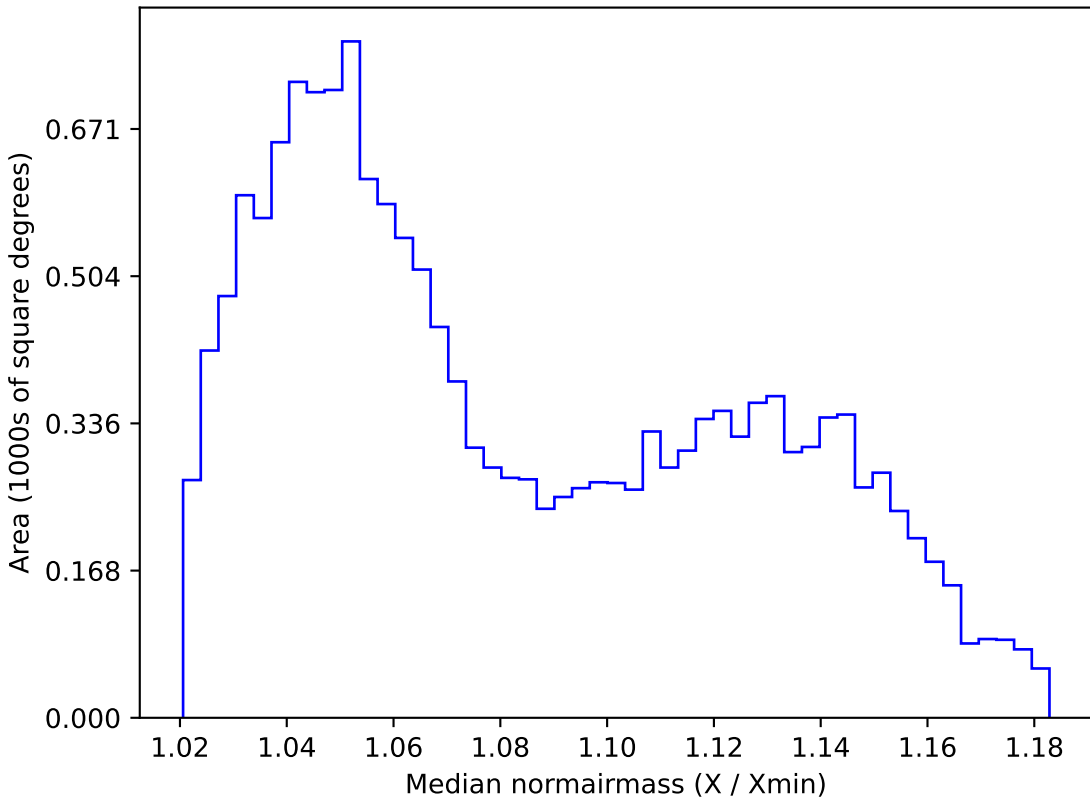
baseline_v3.0_10yrs WFD r band: Median normairmass
