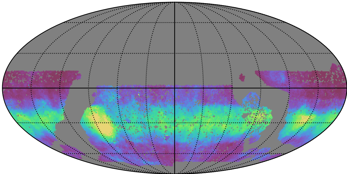
baseline_v3.0_10yrs WFD i band: Median normairmass
