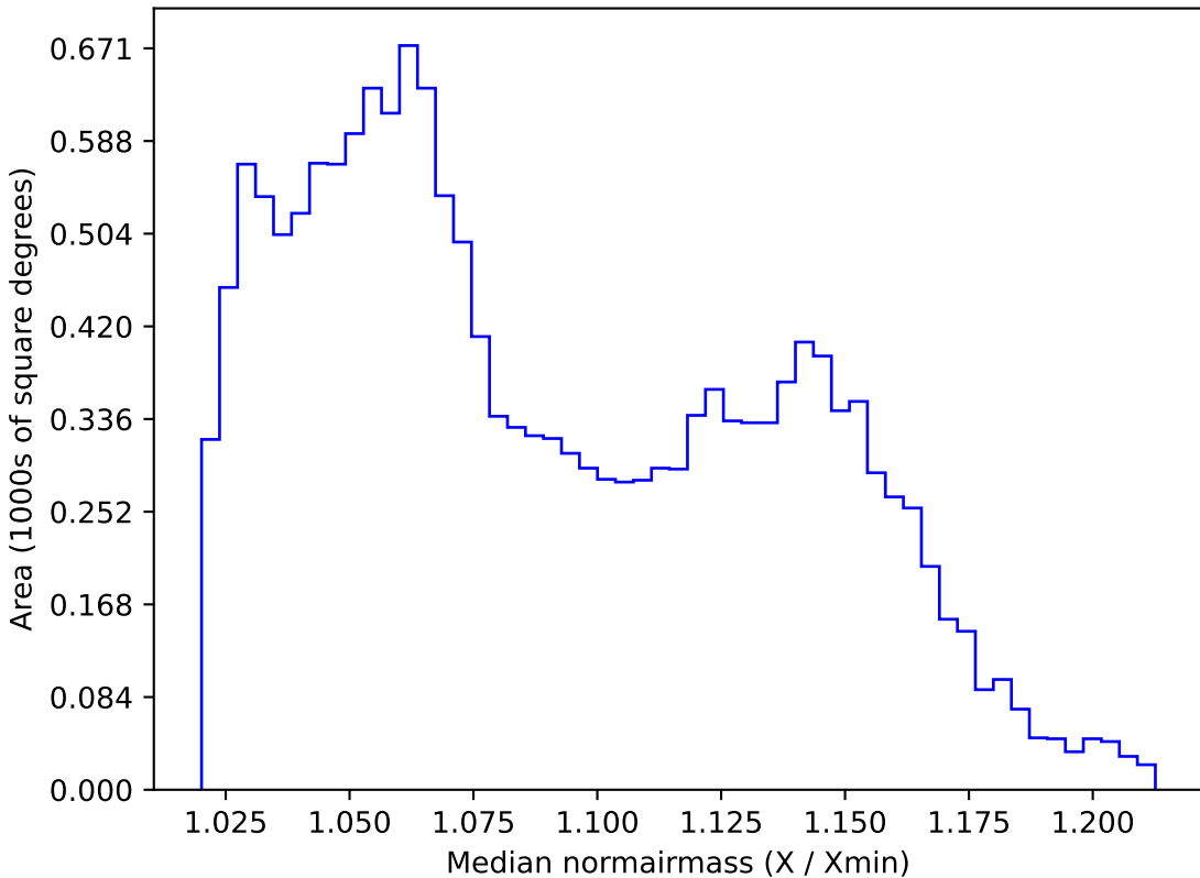
baseline_v3.0_10yrs WFD i band: Median normairmass
