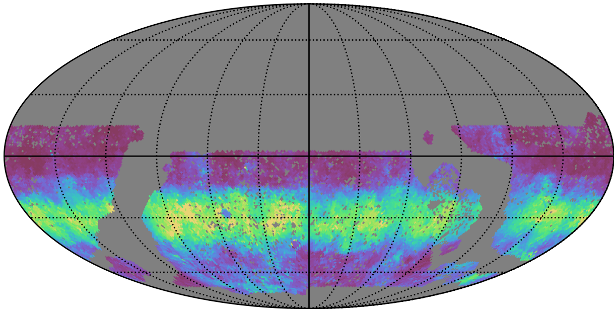
baseline_v3.0_10yrs WFD g band: Median normairmass
