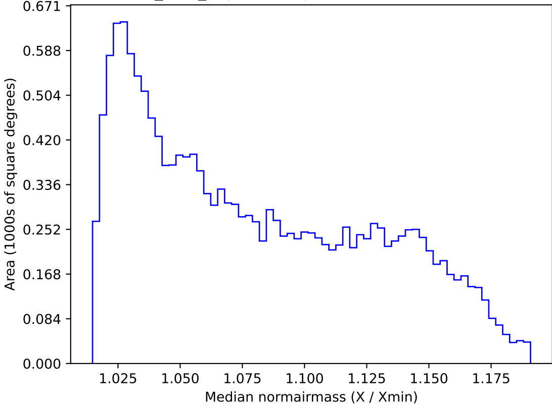
baseline_v3.0_10yrs WFD g band: Median normairmass
