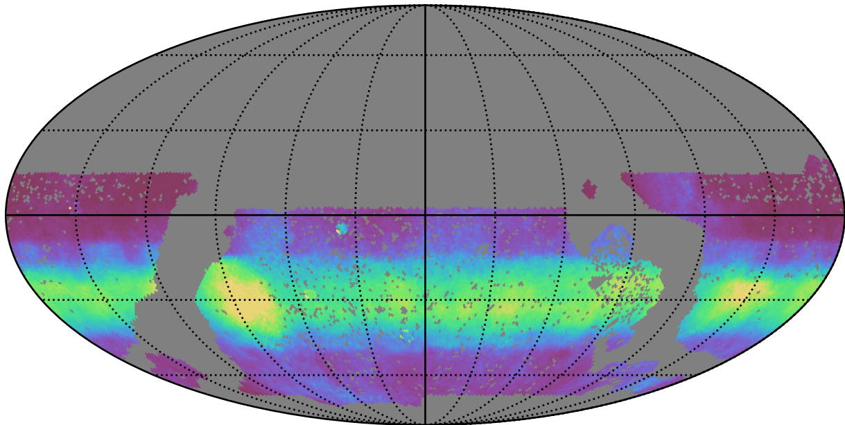
baseline_v3.0_10yrs WFD all bands: Median normairmass
