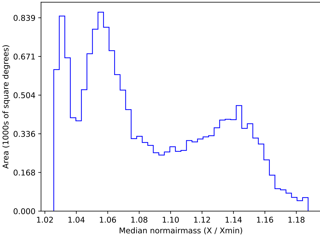
baseline_v3.0_10yrs WFD all bands: Median normairmass
