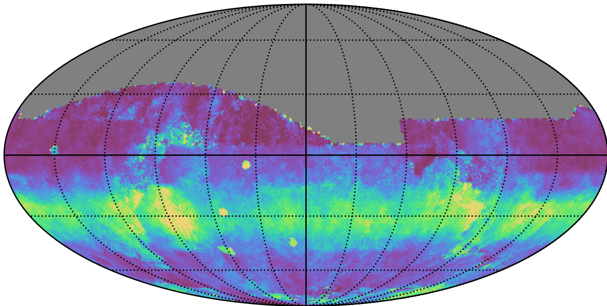
baseline_v3.0_10yrs All sky z band: Median normairmass
