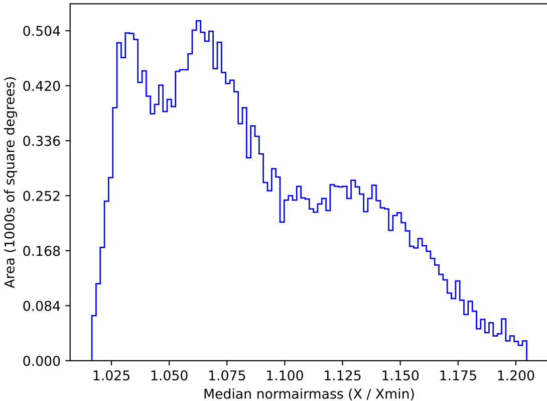
baseline_v3.0_10yrs All sky z band: Median normairmass
