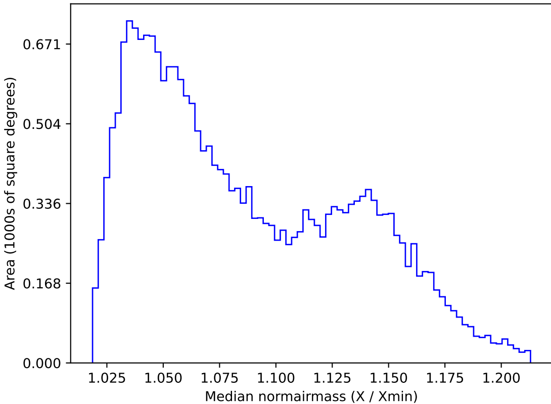
baseline_v3.0_10yrs All sky y band: Median normairmass
