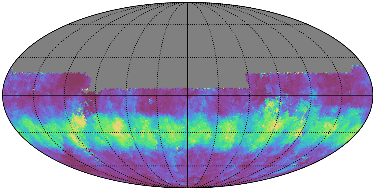
baseline_v3.0_10yrs All sky u band: Median normairmass
