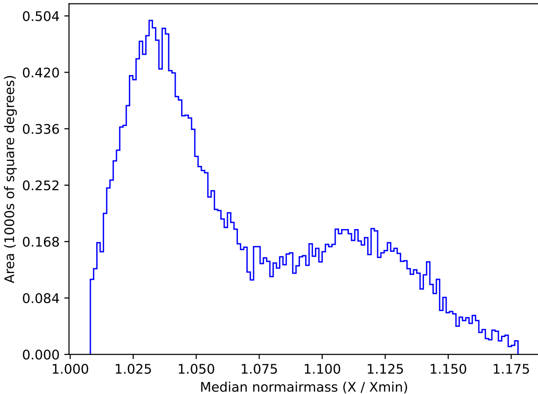
baseline_v3.0_10yrs All sky u band: Median normairmass
