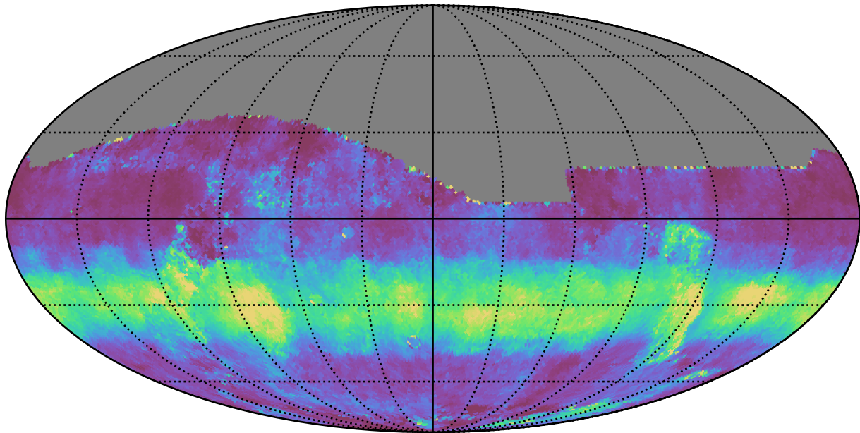
baseline_v3.0_10yrs All sky r band: Median normairmass
