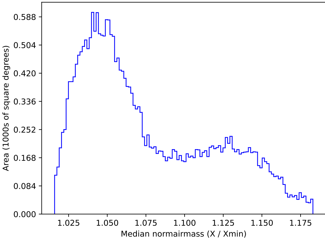
baseline_v3.0_10yrs All sky r band: Median normairmass
