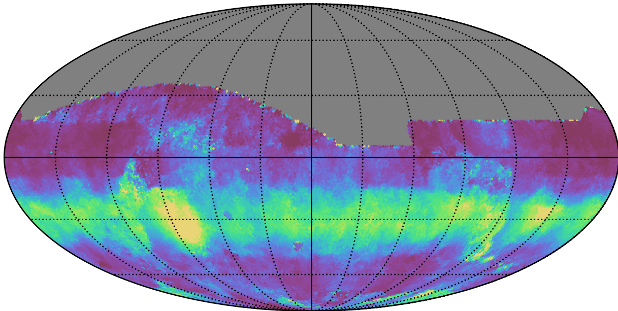
baseline_v3.0_10yrs All sky i band: Median normairmass
