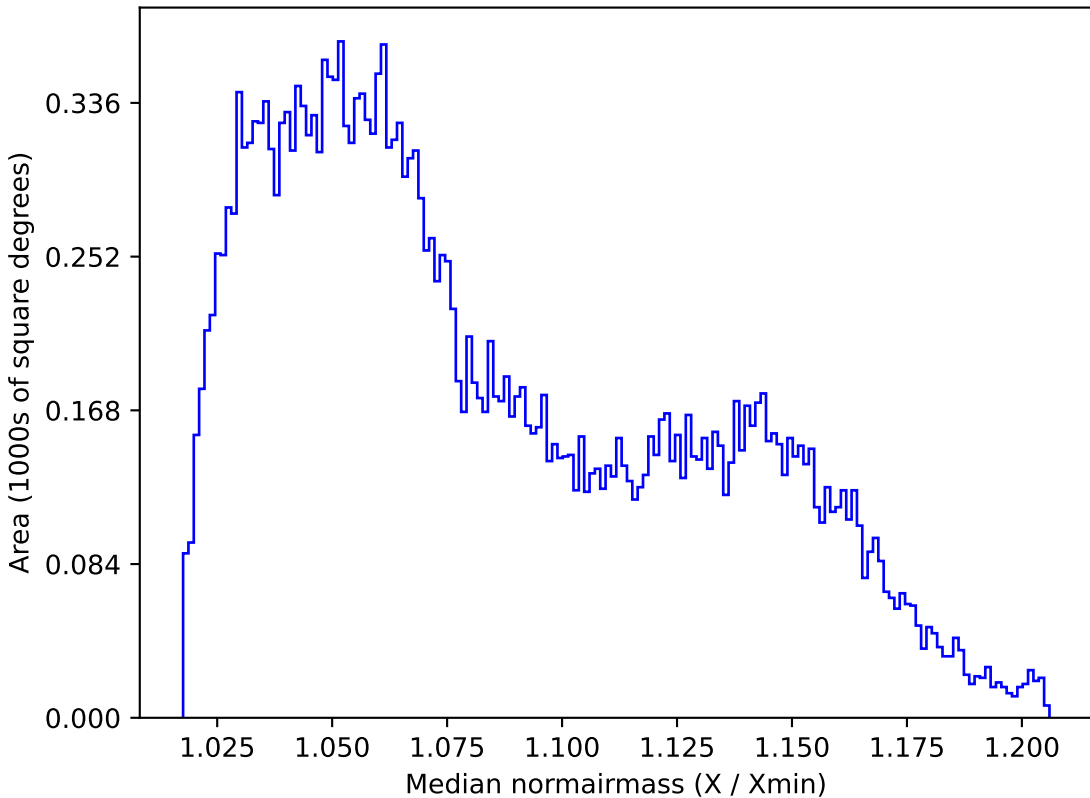
baseline_v3.0_10yrs All sky i band: Median normairmass
