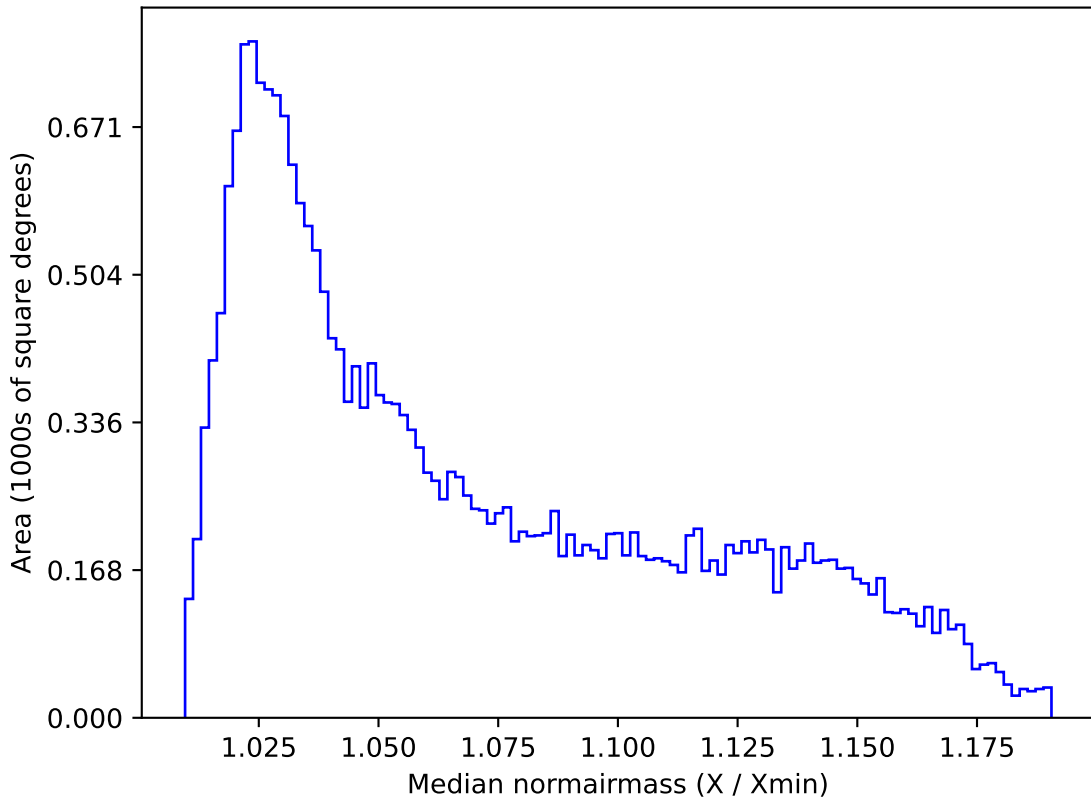
baseline_v3.0_10yrs All sky g band: Median normairmass
