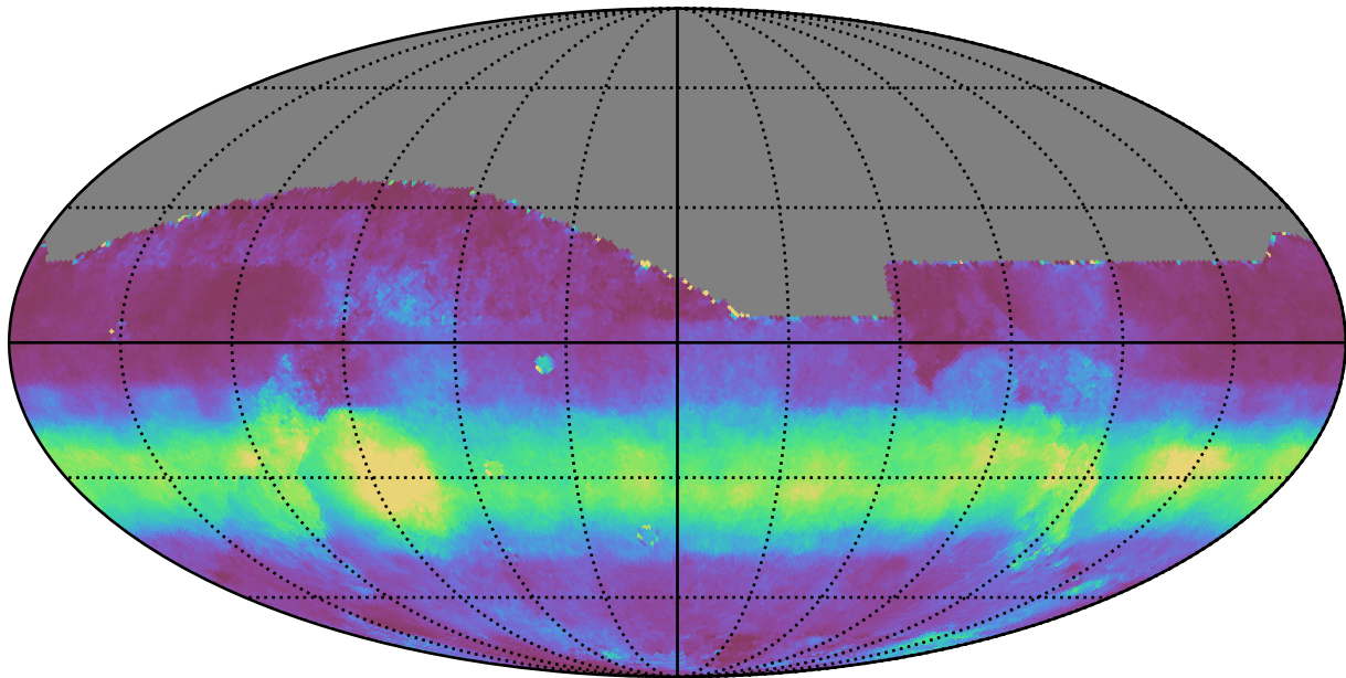
baseline_v3.0_10yrs All sky all bands: Median normairmass
