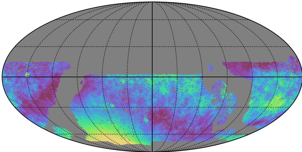
baseline_v3.0_10yrs WFD z band: Median moonDistance
