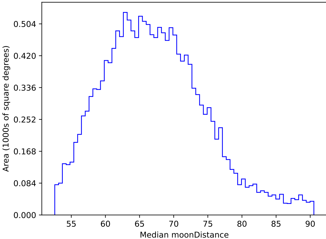
baseline_v3.0_10yrs WFD z band: Median moonDistance
