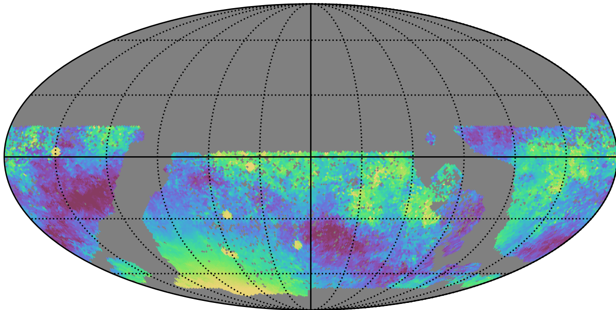
baseline_v3.0_10yrs WFD y band: Median moonDistance
