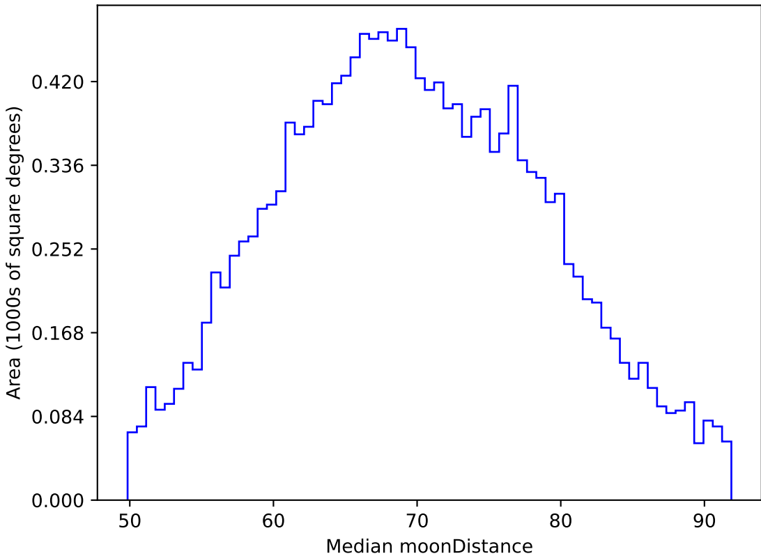
baseline_v3.0_10yrs WFD y band: Median moonDistance
